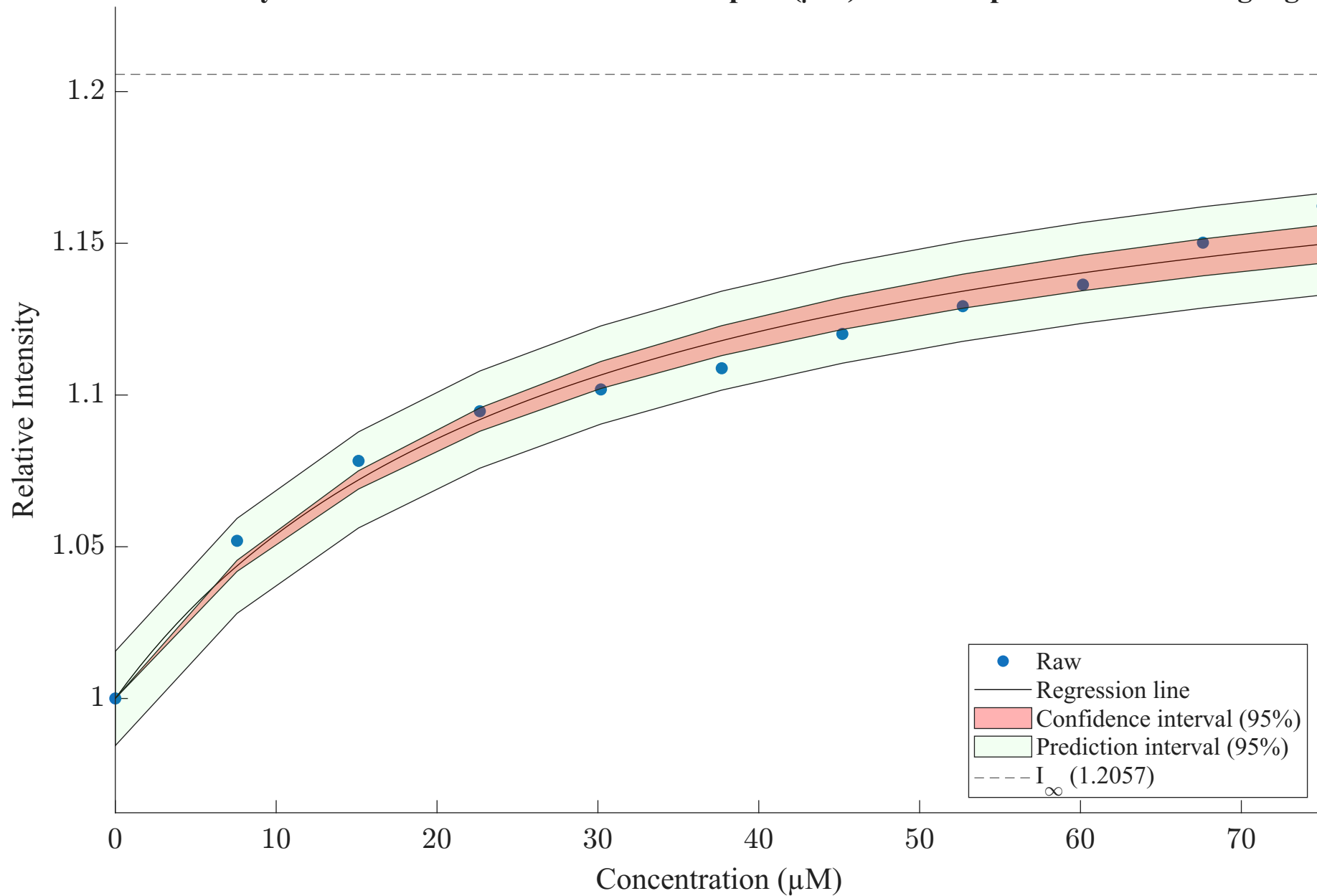
Relative intensity as a function of concentration of lipids ( \mu\text{M} ) for a6r rep3 - Statistics fitting algorithm
